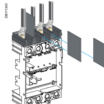
Adapter for 400/630 A - 4P base. Connection with spreaders and interphase barriers.
