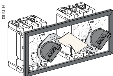
Interlocking of two devices with rotary handles.
